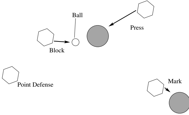
Fig. 1. Defend Actions
