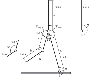
Fig. 12. Planar four-link model of the robot
