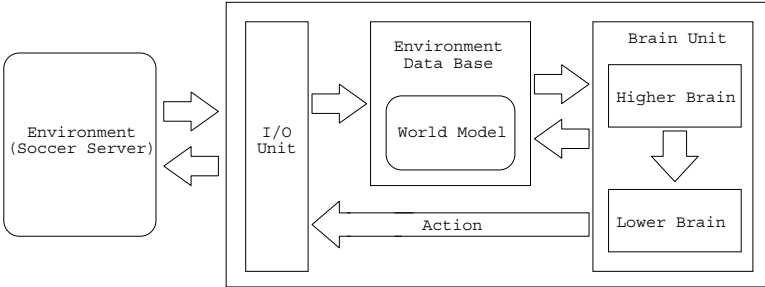
Fig. 1. Agent Architecture
