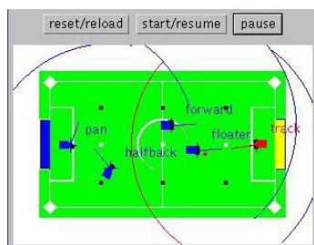
Fig. 3. TeamBots simulation.
