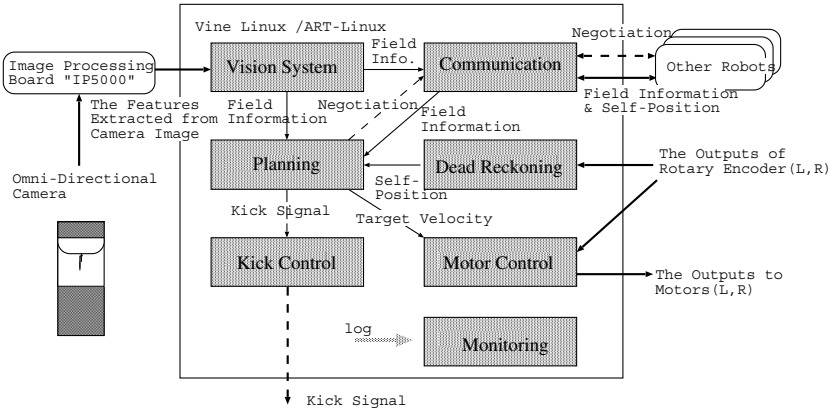
Fig. 3. Software architecture
