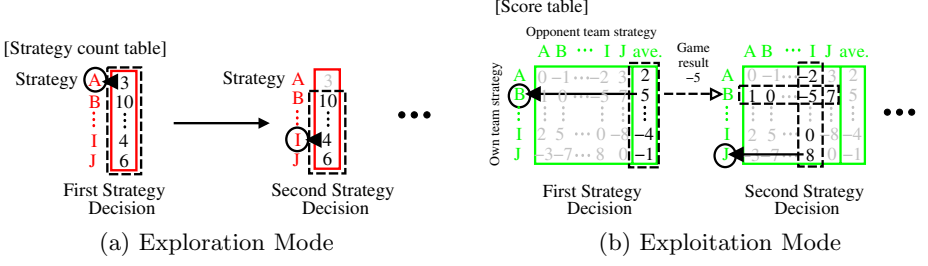
Fig. 1. Strategy selection
