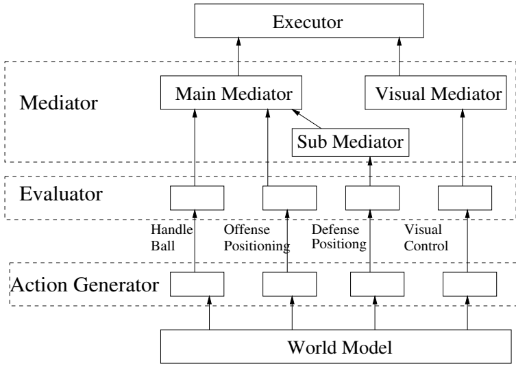
Fig. 2. Strategy Architecture
