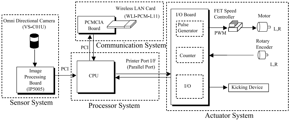
Fig. 2. Hardware architecture
