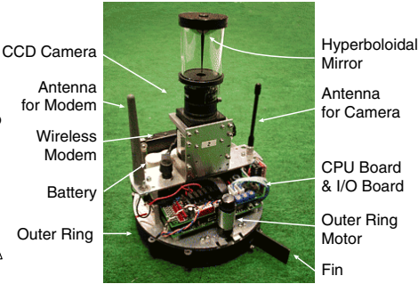
Fig. 1. Concept of the robot system Fig. 2. Overall view of the robot unit
