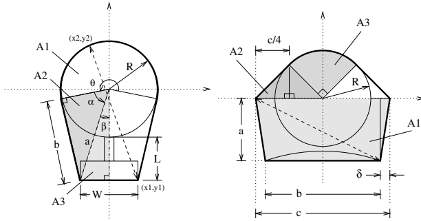
Fig. 2. Diagram showing dimensions used for the convex hull footprint calculation: the central circle denotes the SuperScout platform body while the structure attached below denotes the kicking device fully extended (field robot). Left: field robot; right: goal-keeper robot.
