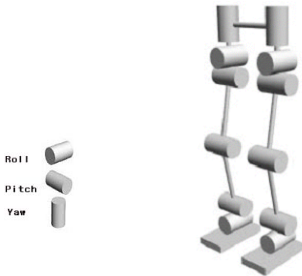
Fig. 1. DOFs configuration
