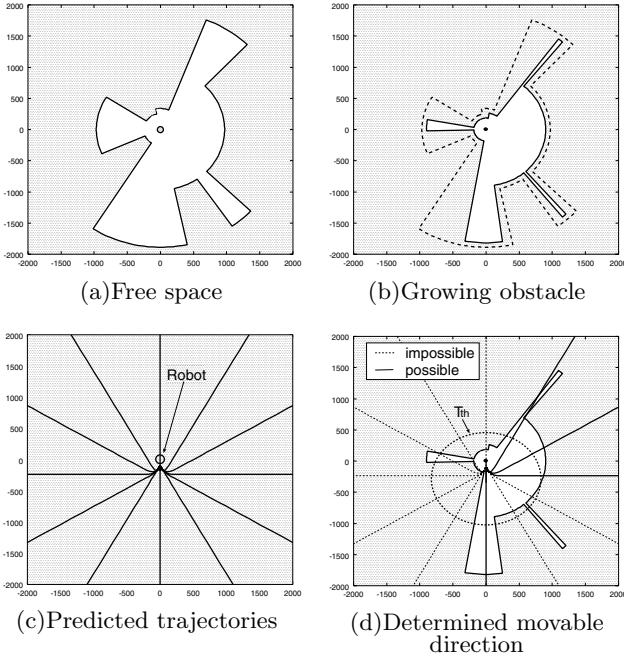
Fig. 4. Example of the method for determining movable direction
