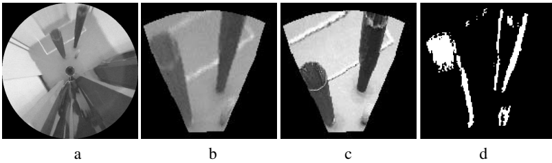
Fig. 3. IPT images acquired by the omni-directional sensor (a) and the standard CCD camera (c). The region of the IPT omnidirectional image corresponding to the field of view of the standard camera (b) and the thresholded difference image (d) are also shown.
