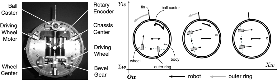
Fig. 4. Concept of the omni-directional mobile mechanism
