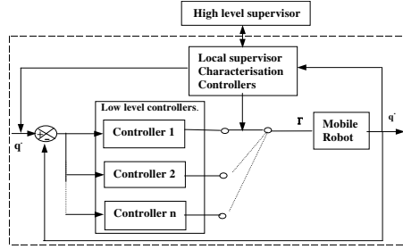
Fig. 2. Hierarchical control structure.
