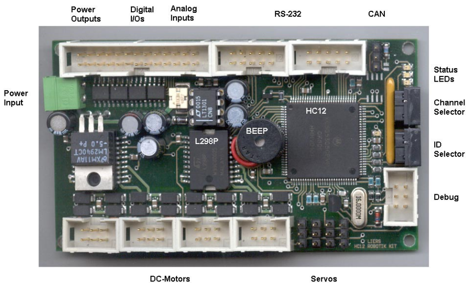
Fig. 2. HC12 microcontroller board.
