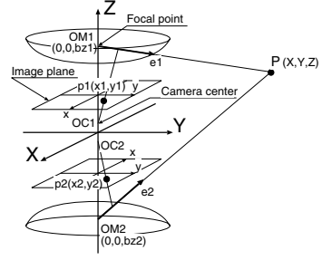
Fig. 4. Camera Coordinate
