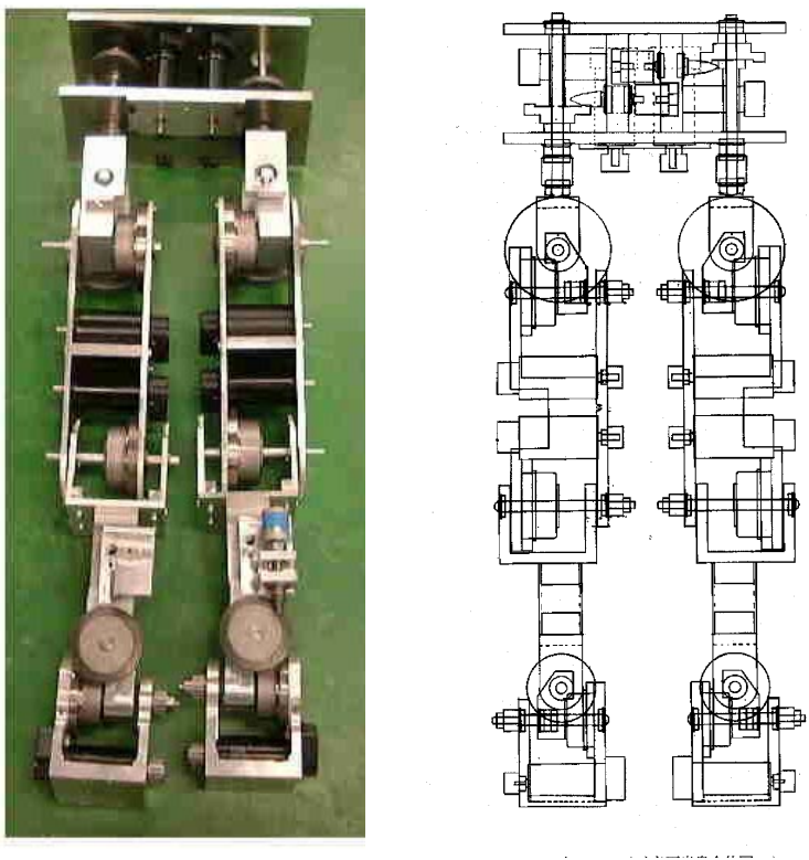
Fig. 2. The mechanical design and a photo of the lower part of KENSEI-chan
