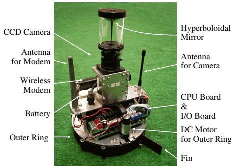
Fig. 1. Overview of the robot
