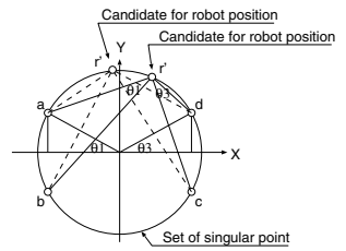
Fig. 8. Singular Points
