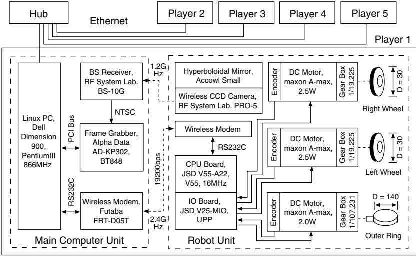
Fig. 3. Configuration of the robot system
