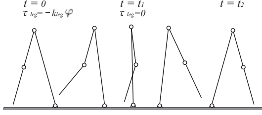
Fig. 3. The motion phases of one cycle
