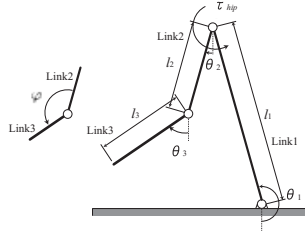
Fig. 2. Planar three link model of the robot
