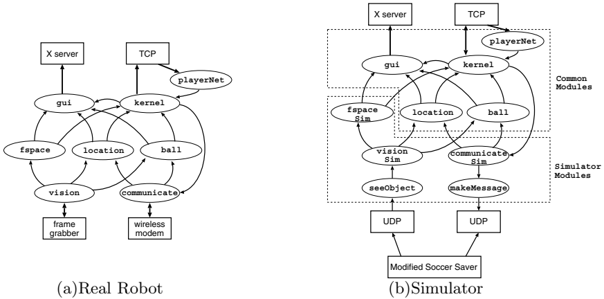
Fig. 5. Configuration of multi-threads
