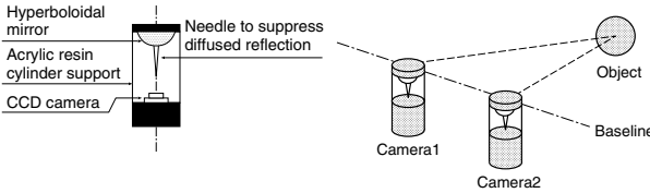
Fig. 1. Omni-Directional Camera
