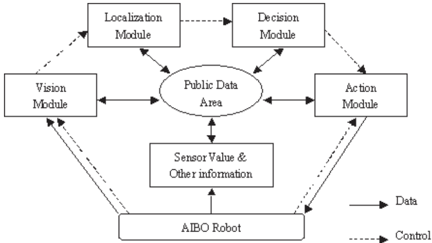
Fig. 1. Architecture of Wright Eagle 2001
