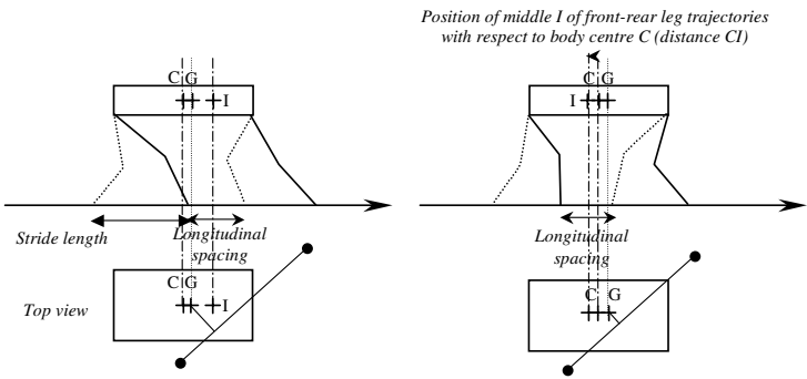
Fig. 1. Position of front-rear leg trajectories in trot. Left: bad configuration that can produce backward fall of the robot. Right: better configuration where trajectories are shifted backwards so that gravity centre is closer to the support diagonal that has just changed.
