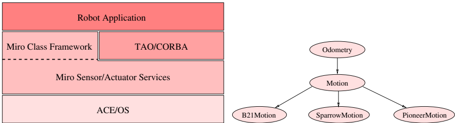
Fig. 1. Left: The Miro Middleware for Robots. Right: Motion interface inheritance for different mobile bases.
