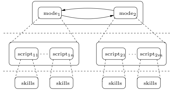
Fig. 1. Three-level approach.
