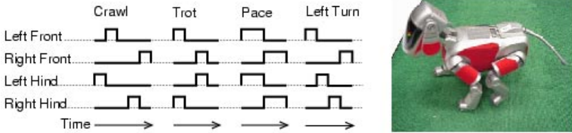
Fig. 1. A timing diagram of various walking gaits. the function is zero when the foot is on the ground and nonzero when it is in the air. To the right is a picture of a robot executing a crawl gait.
